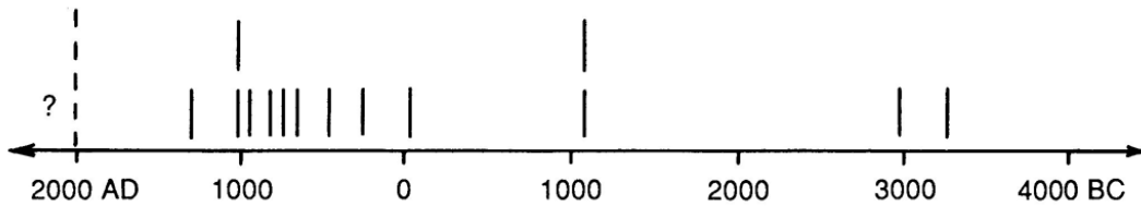
Figure 5. History of minor Galactic Center explosions during the past 6000 years; dates approximate times when radiation pulses arrived from the Galactic Center. (These age estimates taken from Lacy et al., (27) have been decreased by, ~70% to correct for the smaller value of 23,000 light years adopted here for the distance to the center of the Galaxy. (4) ) © 1989 P. LaViolette
