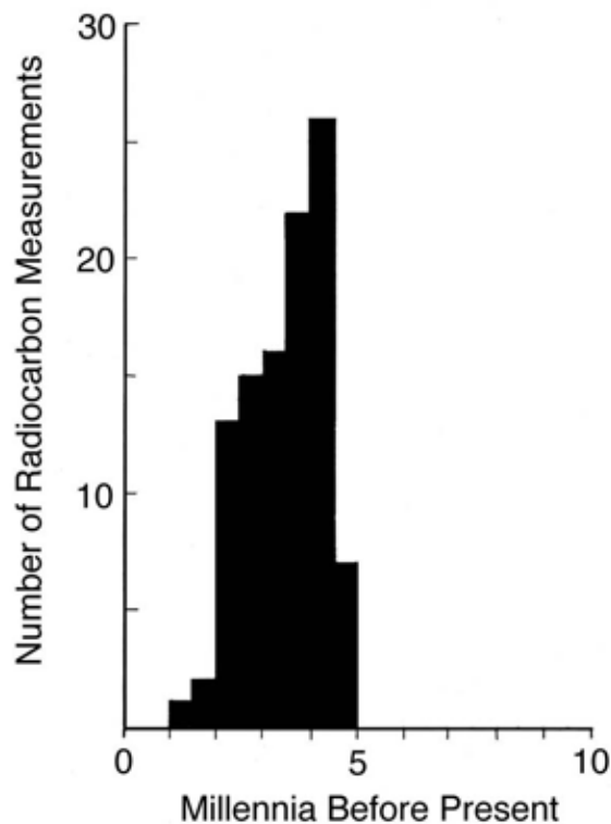
Figure 4. Histogram showing the number of published radiocarbon dates from the lower Nile valley for each of a series of calendar year increments. (26)
