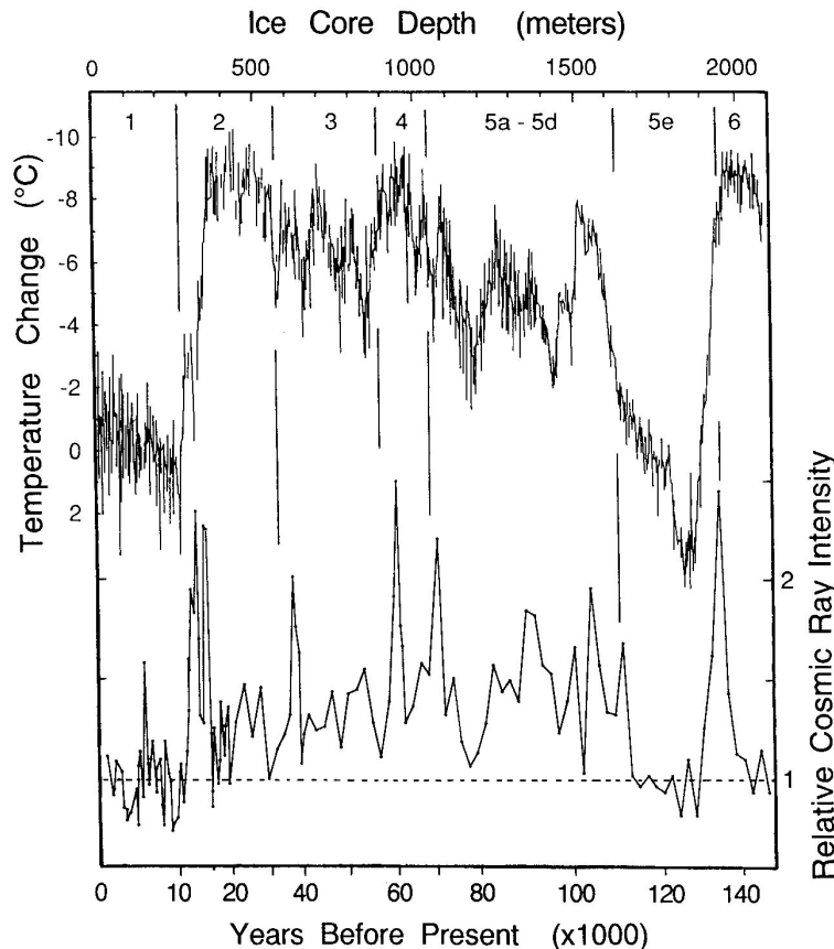
Figure 3. The lower graph plots cosmic ray intensity variations at the Earth's surface during the past 145,000 years; see The Talk of the Galaxy . (21) These values were derived from beryllium-10 isotope concentrations found in the Vostok (East Antarctica) ice core (22-23) that were adjusted to correct for variations in ice accumulation rate and solar activity. The upper graph plots global climate. The numbered climatic zones include: the present interglacial (1), the last ice age (2, 3, & 4), a semiglaciated interval (5a-d), the last interglacial (5e), and the previous glaciation (6).
