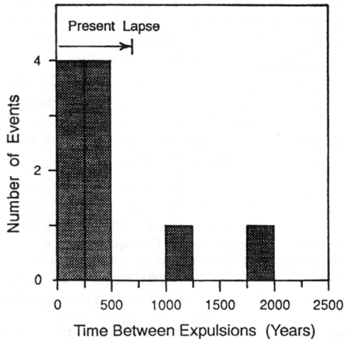
Figure 6. Amount of time between successive gas expulsions from the Galactic center, plotted as a frequency histogram. © 1989 P. LaViolette
